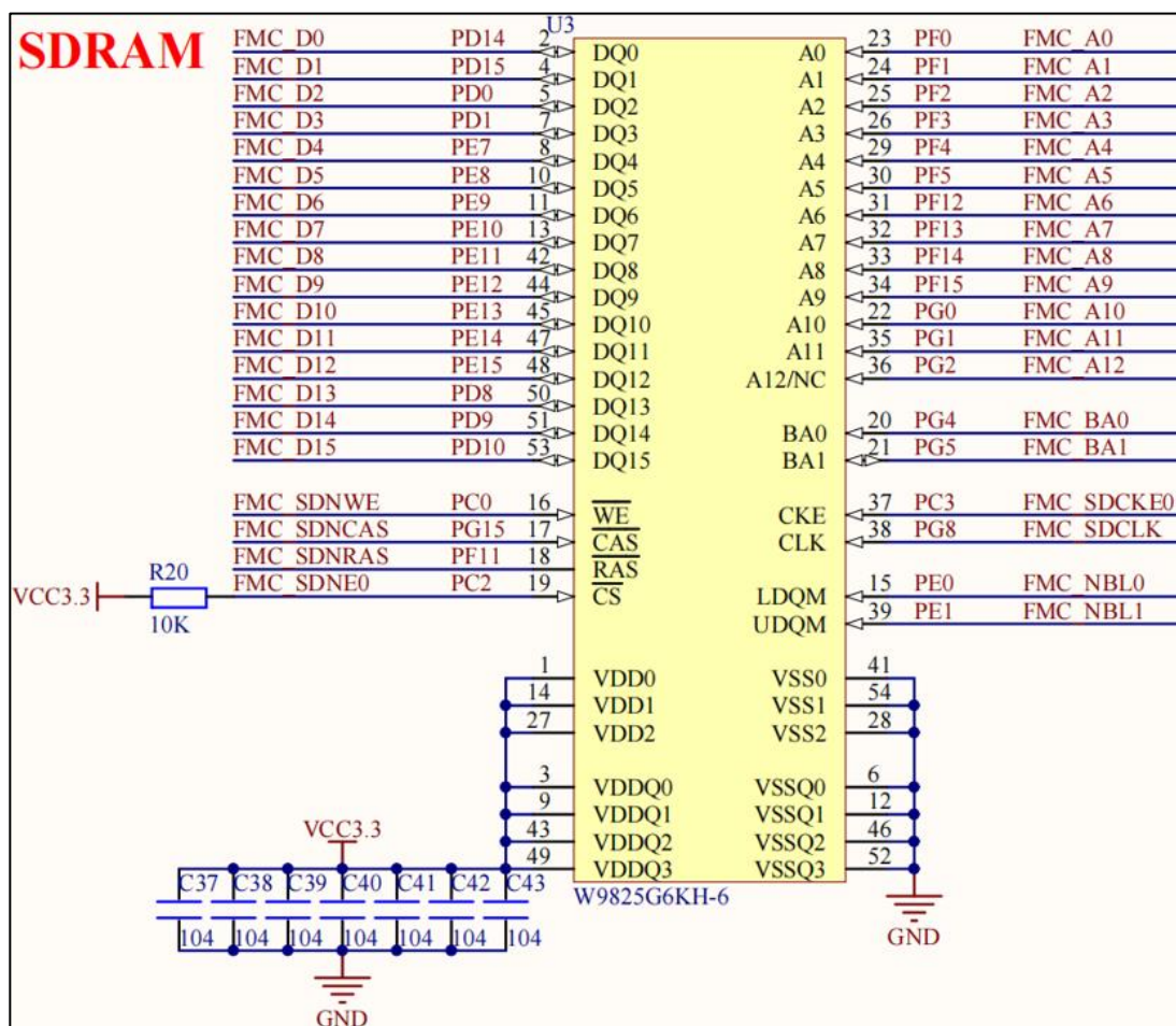
2.2.4.1 SDRAM
