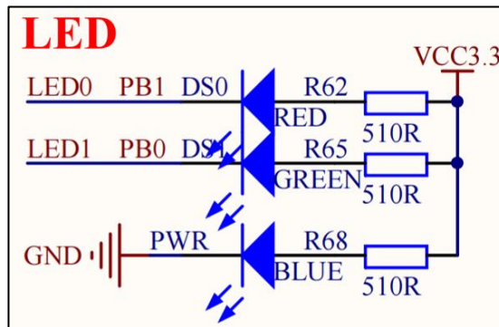
图 2.1.20.1 LED
