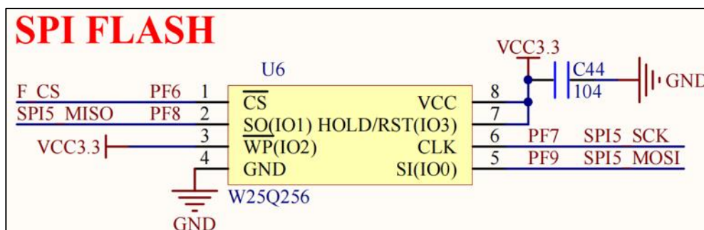
2.2.6.1 SPI FLASH
